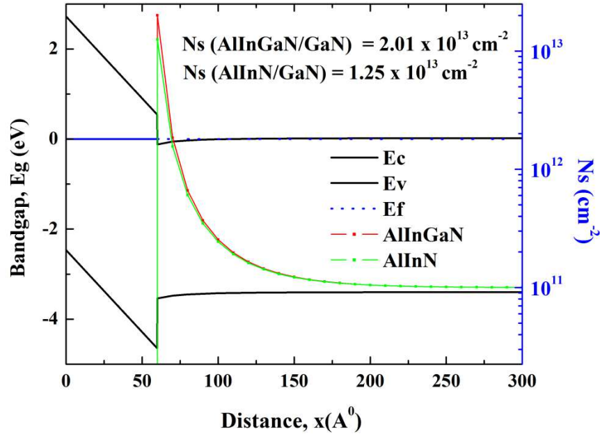
Figure 6.4: Self-consistent Poisson Schrödinger simulation of an LM-AlInN/GaN and AlInGaN/GaN heterostructure using the software BandEng [125]. The conduction band and the valence band profile as well as the sheet carrier concentration are shown.
