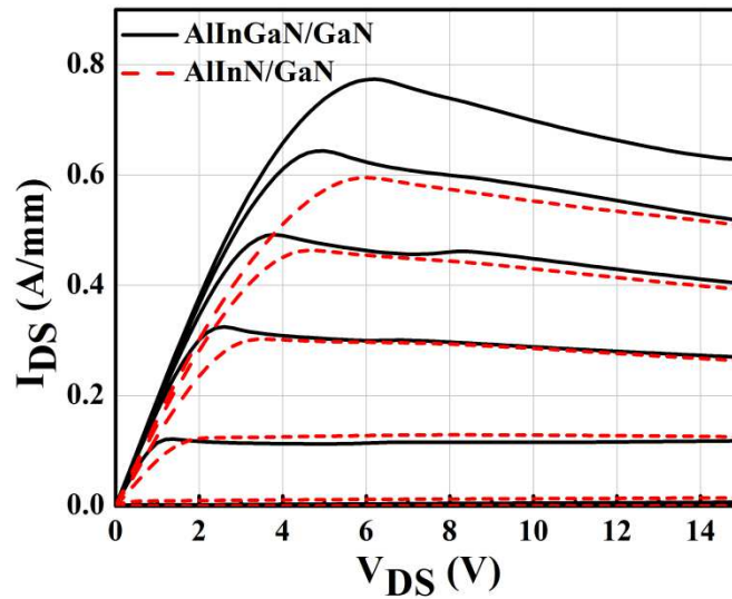
Figure 6.6: Typical static output I-V characteristics of a 1.8 \times 100 \mu\text{m}^2 standard AlInN/GaN MOSHEMT and AlInGaN/GaN MOSHEMT for V_{gs\text{max}} = +2\text{V} with -1\text{V} step size.
