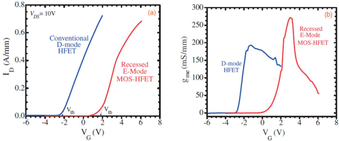
Figure 4.4 : RT transfer characteristics (a) and extrinsic transconductance (b) of identical geometry AlInN/GaN D-mode HFET and E-mode insulating-gate HFET processed from the wafer. V_{DS} = 10\text{ V} .
