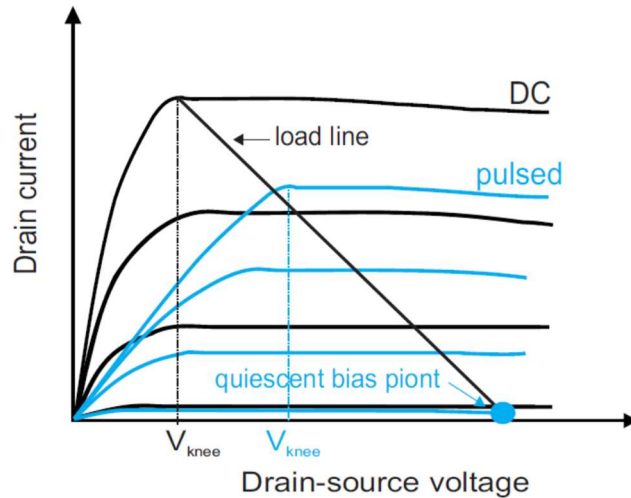
Figure 2.11: Typical DC and pulsed I-V characteristics of an AlGaN/GaN HFET. The pulsed I-V curves are measured at a special quiescent bias point marked by the blue circle.
