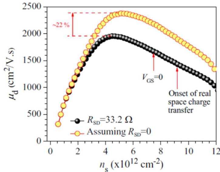
Figure 5.6: Sheet carrier density dependence of the drift mobility derived from the channel conductance measurements for a fat-gate MOSHEMT ( L_G = 60 \mu\text{m} ) and corrected for the series resistance effects.
